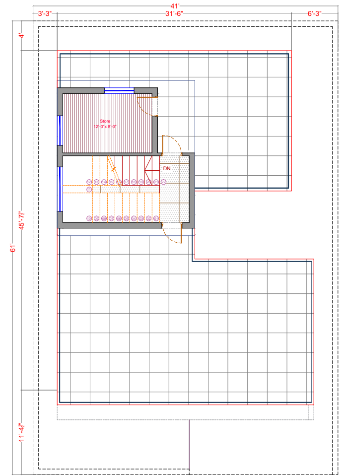
03 TERRACE FLOOR PLAN 278 Sq yds east facing villa
