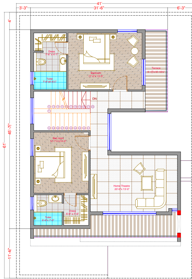
02 FIRST FLOOR PLAN 278 Sq yds east facing villa
