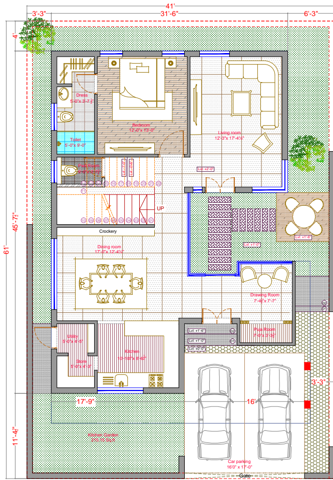
01 GROUND FLOOR PLAN 278 Sq yds east facing villa
